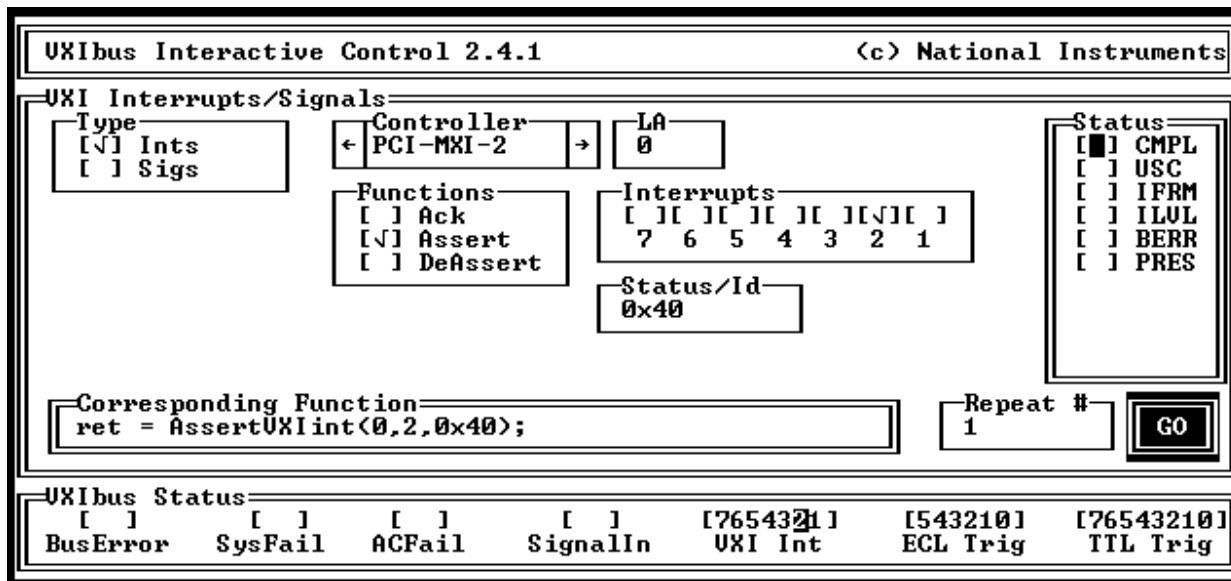
Figure 4-4. Interrupt Utility
